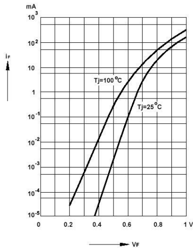
Forward characteristics
