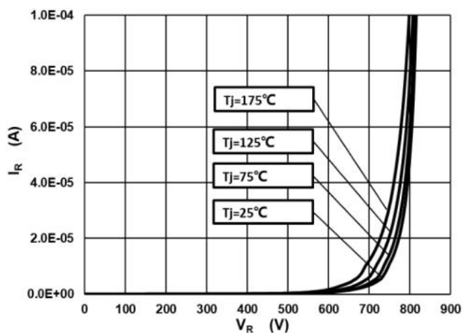
Fig.2 –Reverse Characteristics
