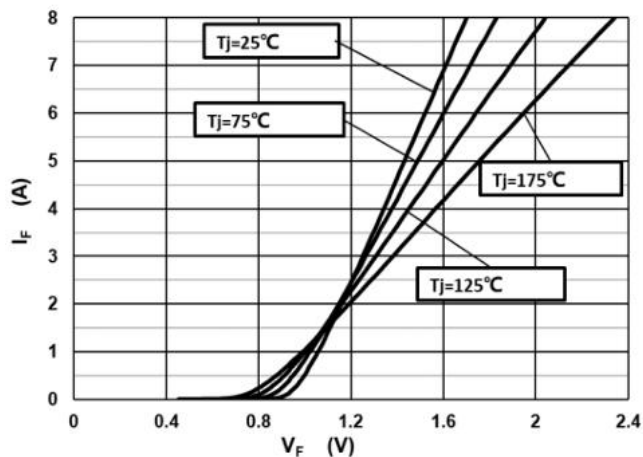
Fig.1 –Forward Characteristics
