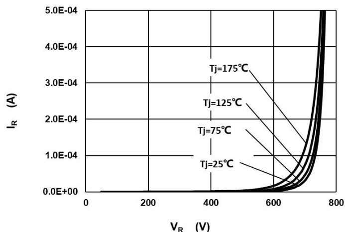
Fig.2 –Reverse Characteristics
