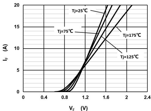
Fig.1 –Forward Characteristics
