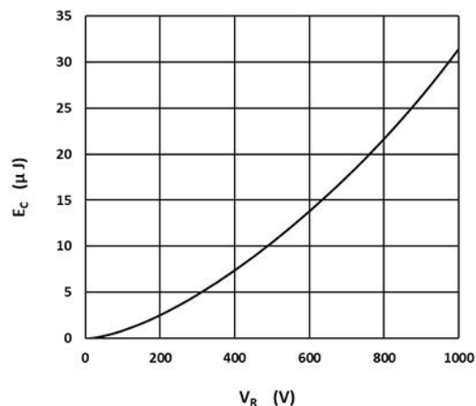
Fig.6 –Typical Capacitance Stored Energy
