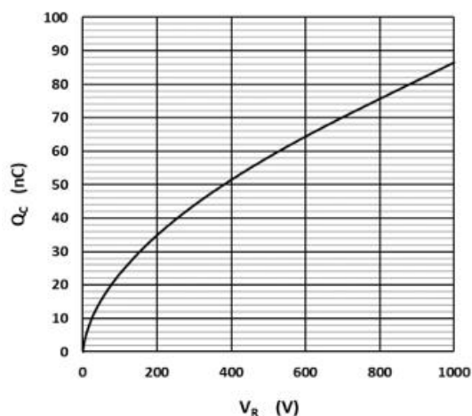
Fig.5 –Total Capacitance Charge vs. Reverse Voltage
