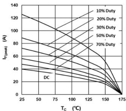
Fig.3 –Current Derating
