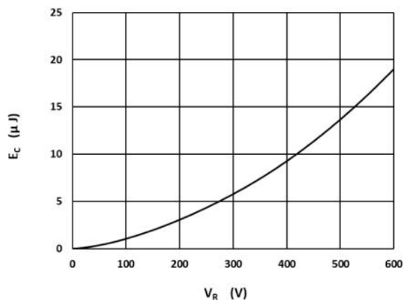
Fig.6 –Typical Capacitance Stored Energy
