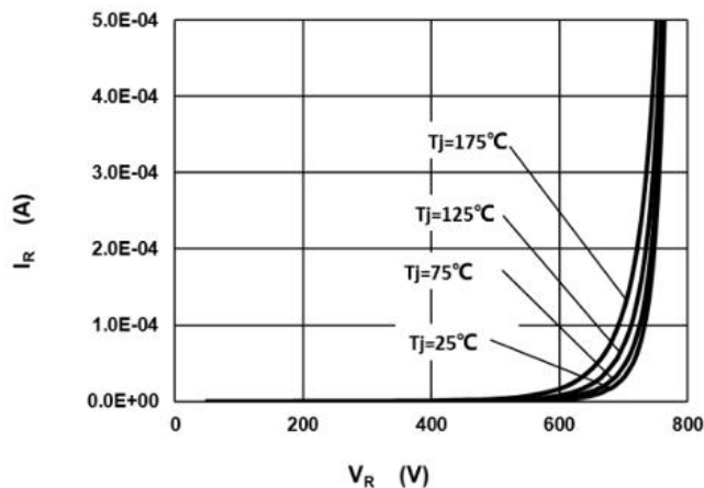
Fig.2 –Reverse Characteristics
