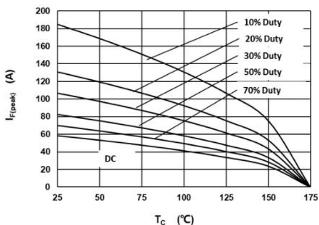
Fig.3 –Current Derating
