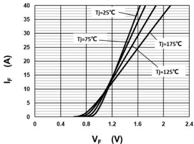
Fig.1 –Forward Characteristics
