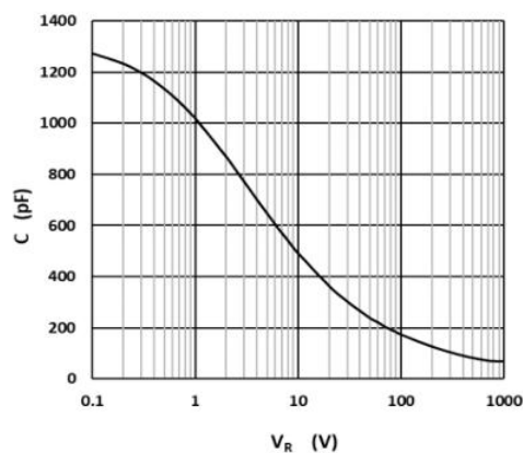
Fig.2 –Reverse Characteristics
